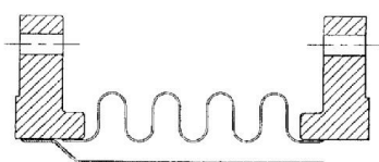
Detalle de Camisa interior / Inner Sleeve detail
